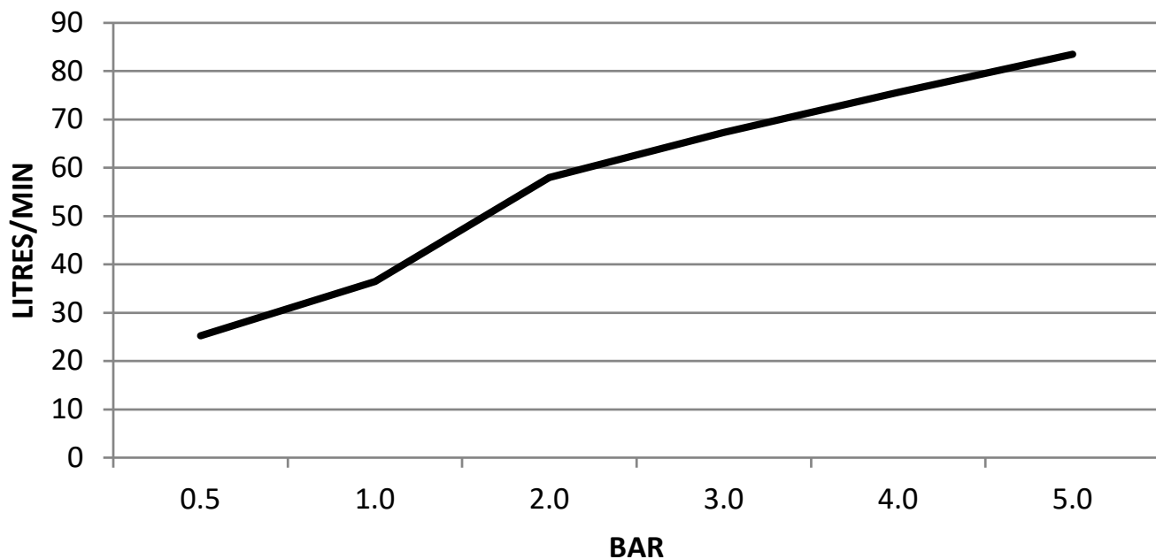
T1146 FLOW RATE LITRES/MIN
