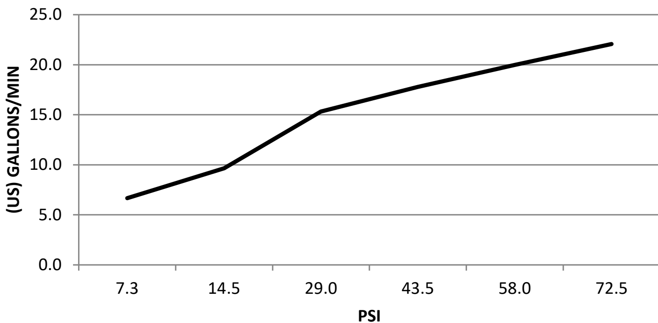
T1146 FLOW RATE (US) GALLONS/PSI
