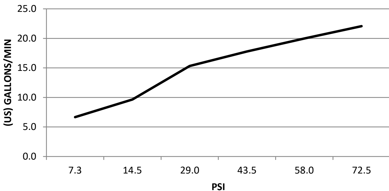
T11K47 FLOW RATE (US) GALLONS/PSI
