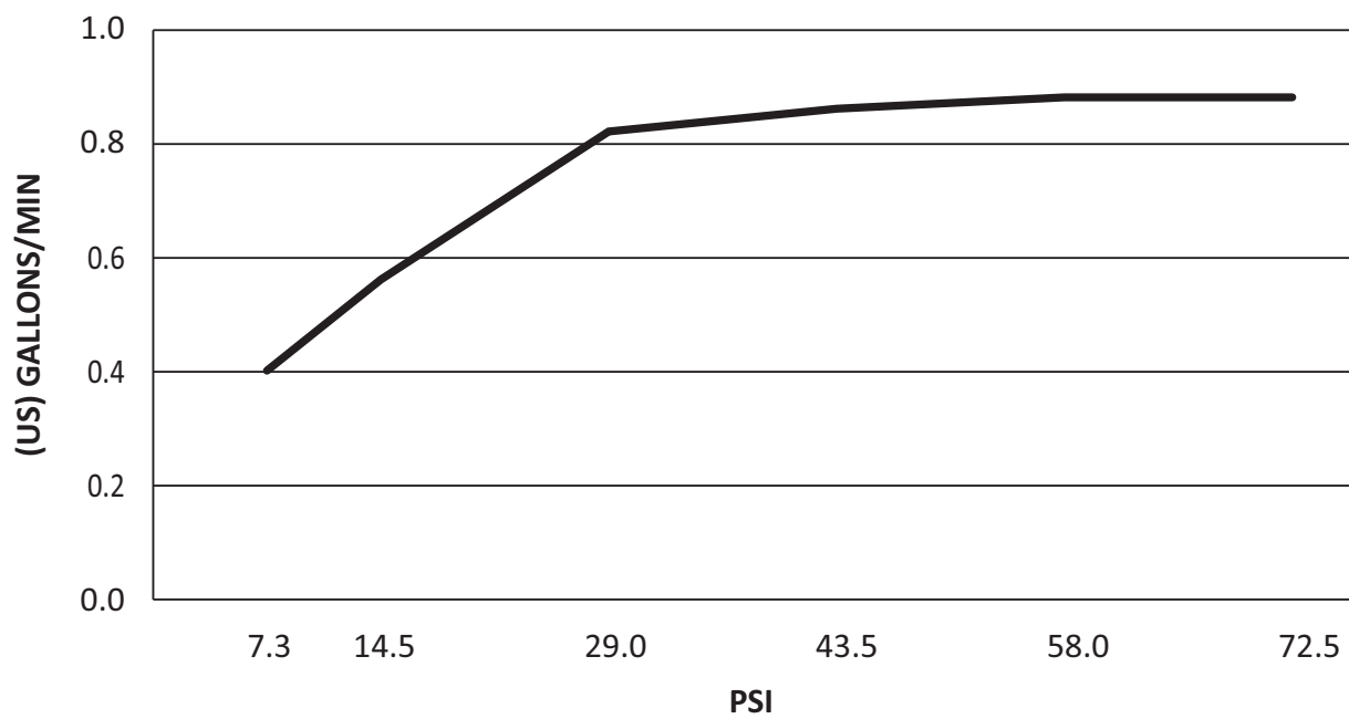
T1114/15/16 FLOW RATE (US) GALLONS/PSI
