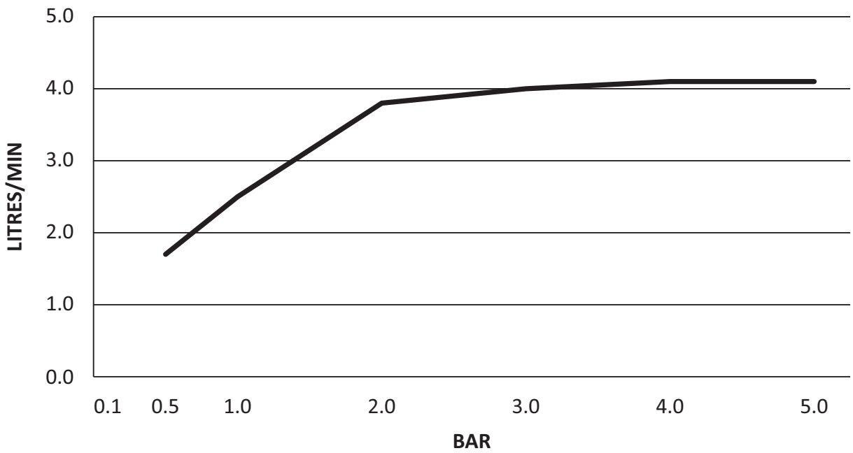
T1114/15/16 FLOW RATE LITRES/MIN
