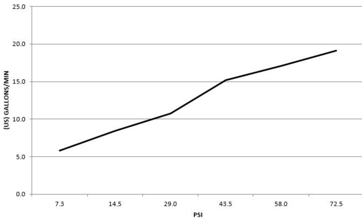
T20K42 FLOW RATE (US) GALLONS/PSI
