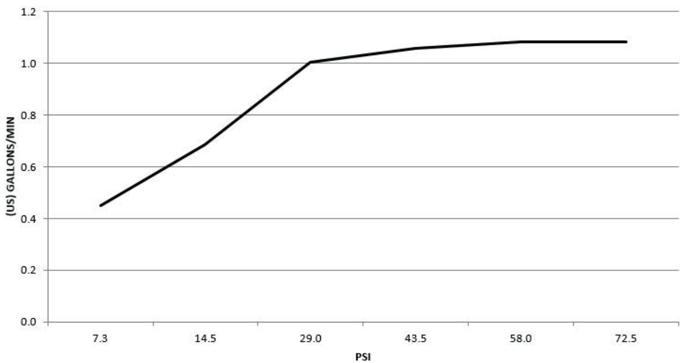
V7K09 / V7K10 FLOW RATE (US) GALLONS/PSI
