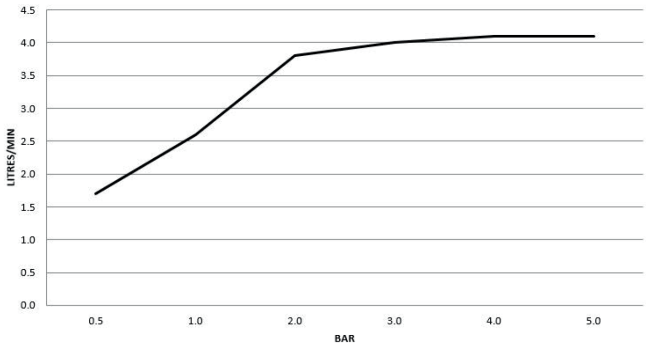
V7K09/ V7K10 FLOW RATE LITRES/MIN
