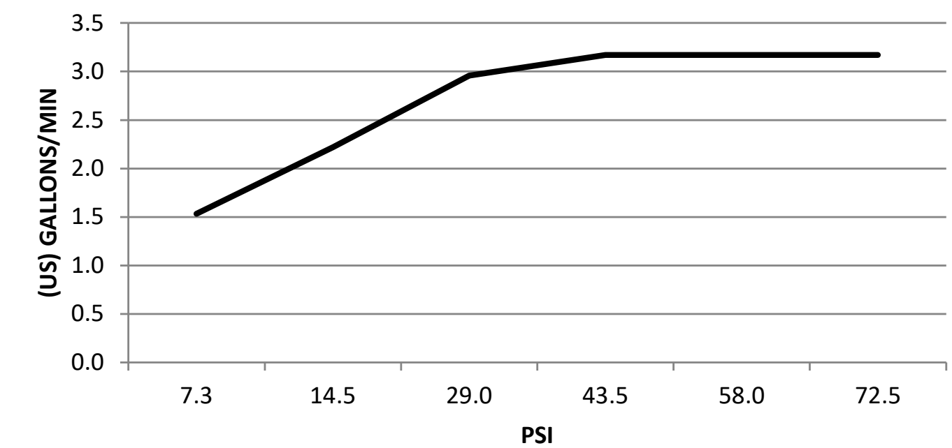
V378 FLOW RATE (US) GALLONS/PSI
